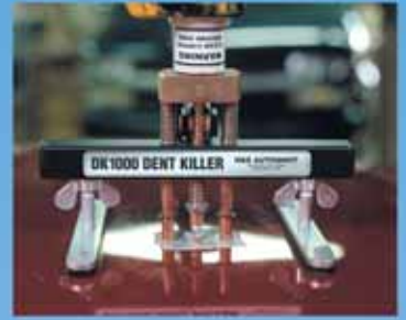
The Dent Killer is welded to the panel surface using a UNI-SPOTTER Stud Welder.
