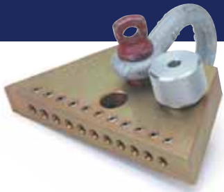
1080 Uni-Clamp multiple stud puller Parts: 1081 - screws only, pkg of 8 1082 - screw wrench only
